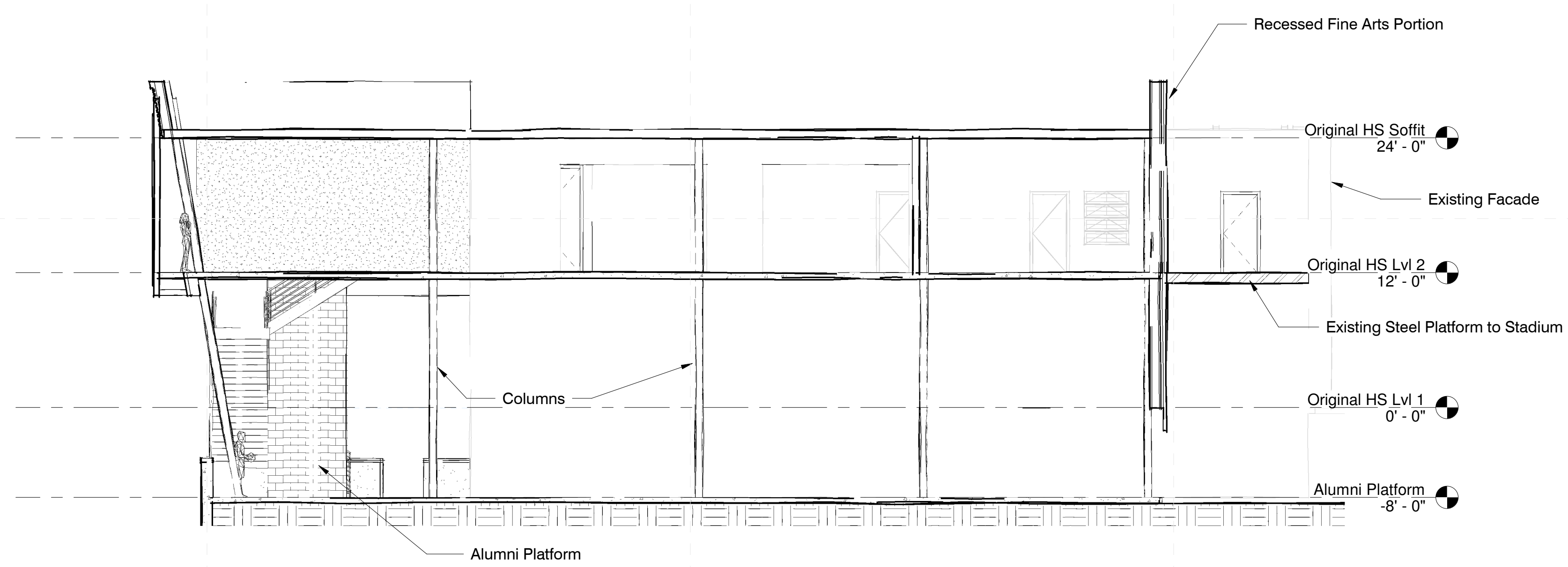
1 Sketch - Section at Fine Arts 1/8" = 1'-0"
