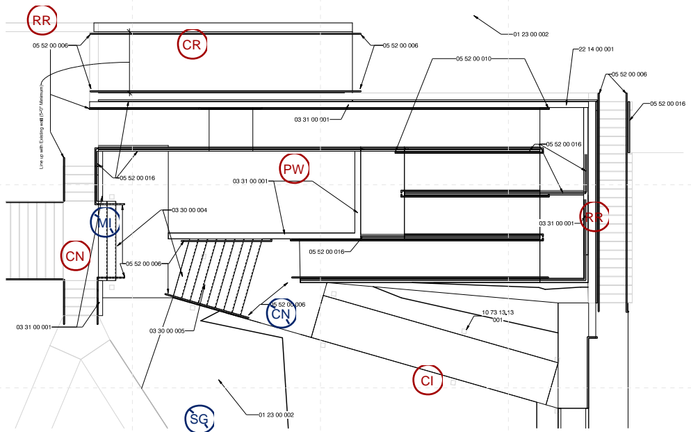
3 PCS Site ADA - Upper Site Ramp 1/4" = 1'-0"
