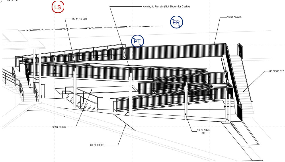
2 Isometric Drawing
