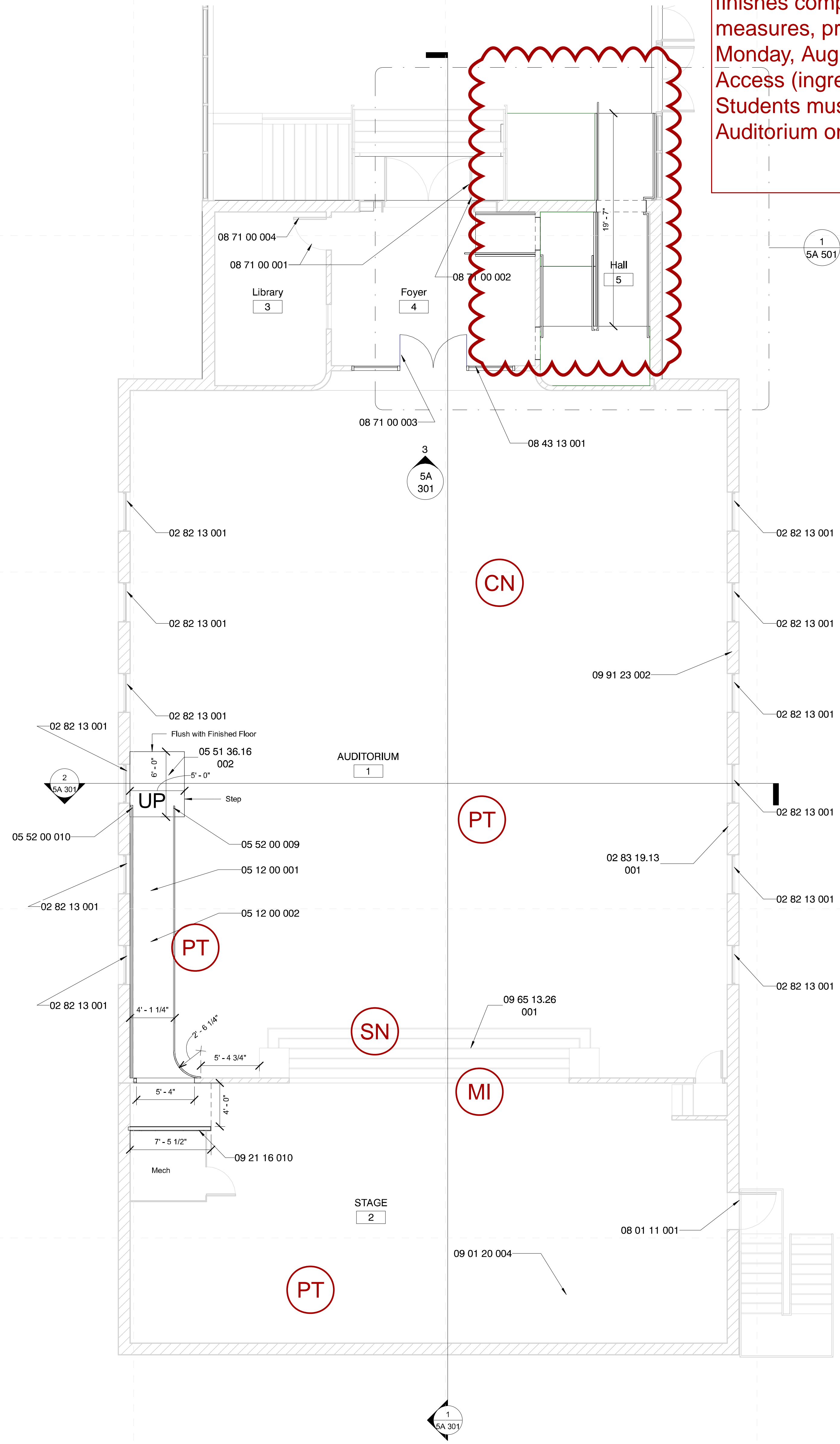
1 PCS Middle - Auditorium - New Construction 3/16" = 1'-0"
