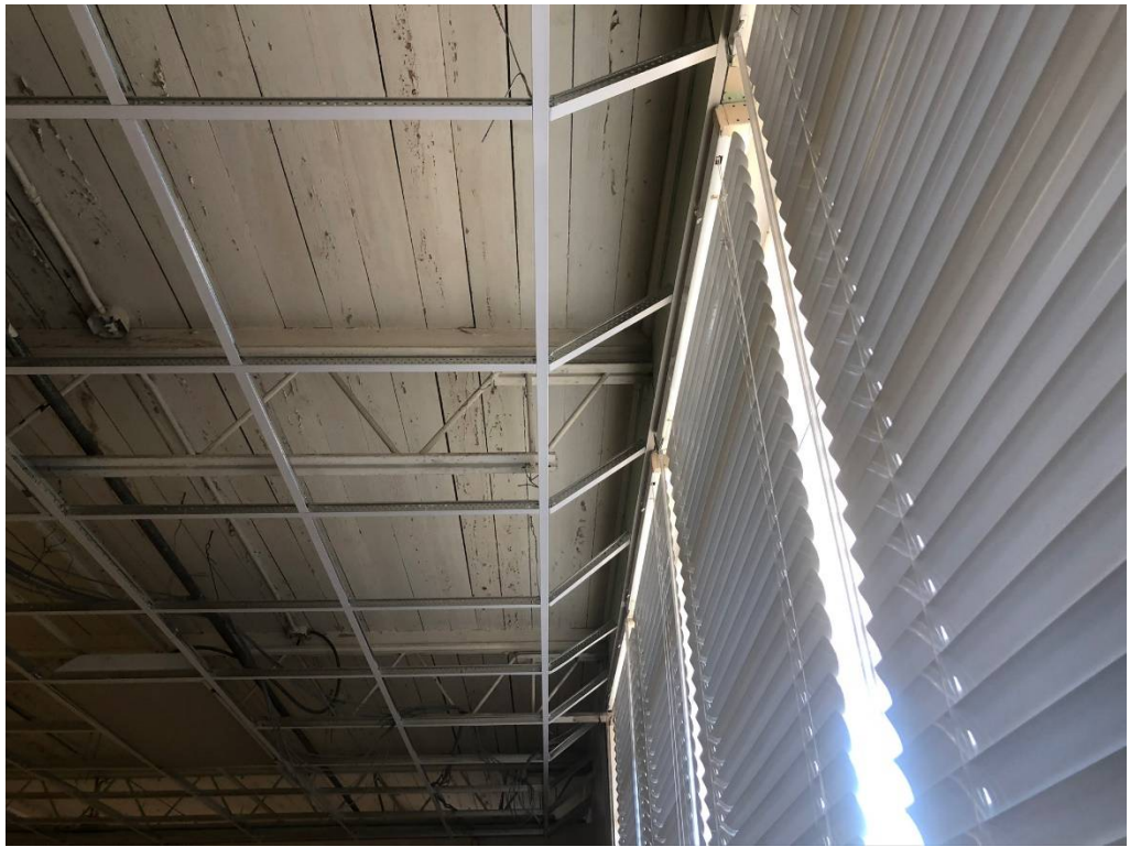
Figure 3 – Typical Detail at High Windows
