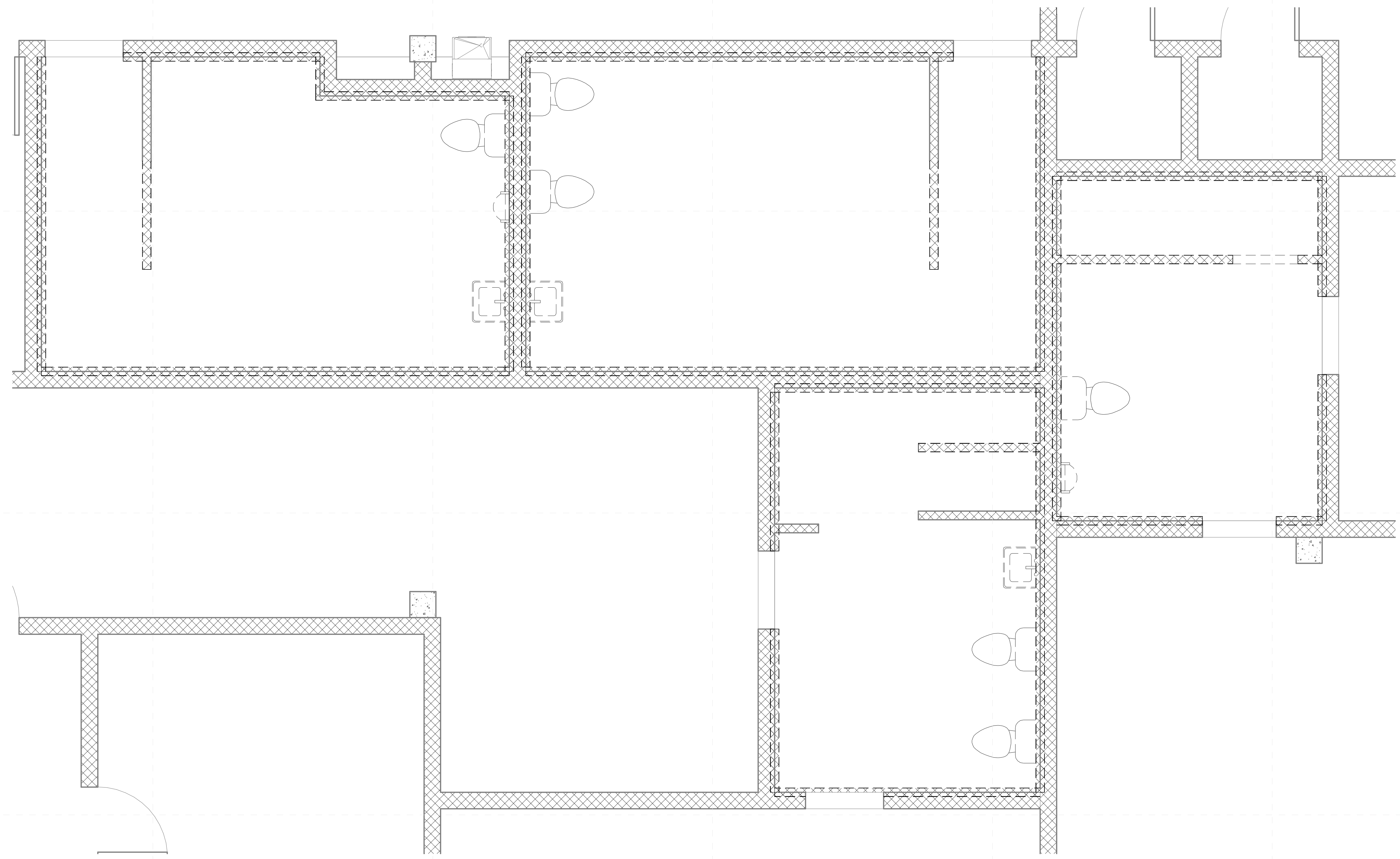
1 PCS Junior High 1st LVL - Bathrooms DEMO 1/2" = 1'-0"
