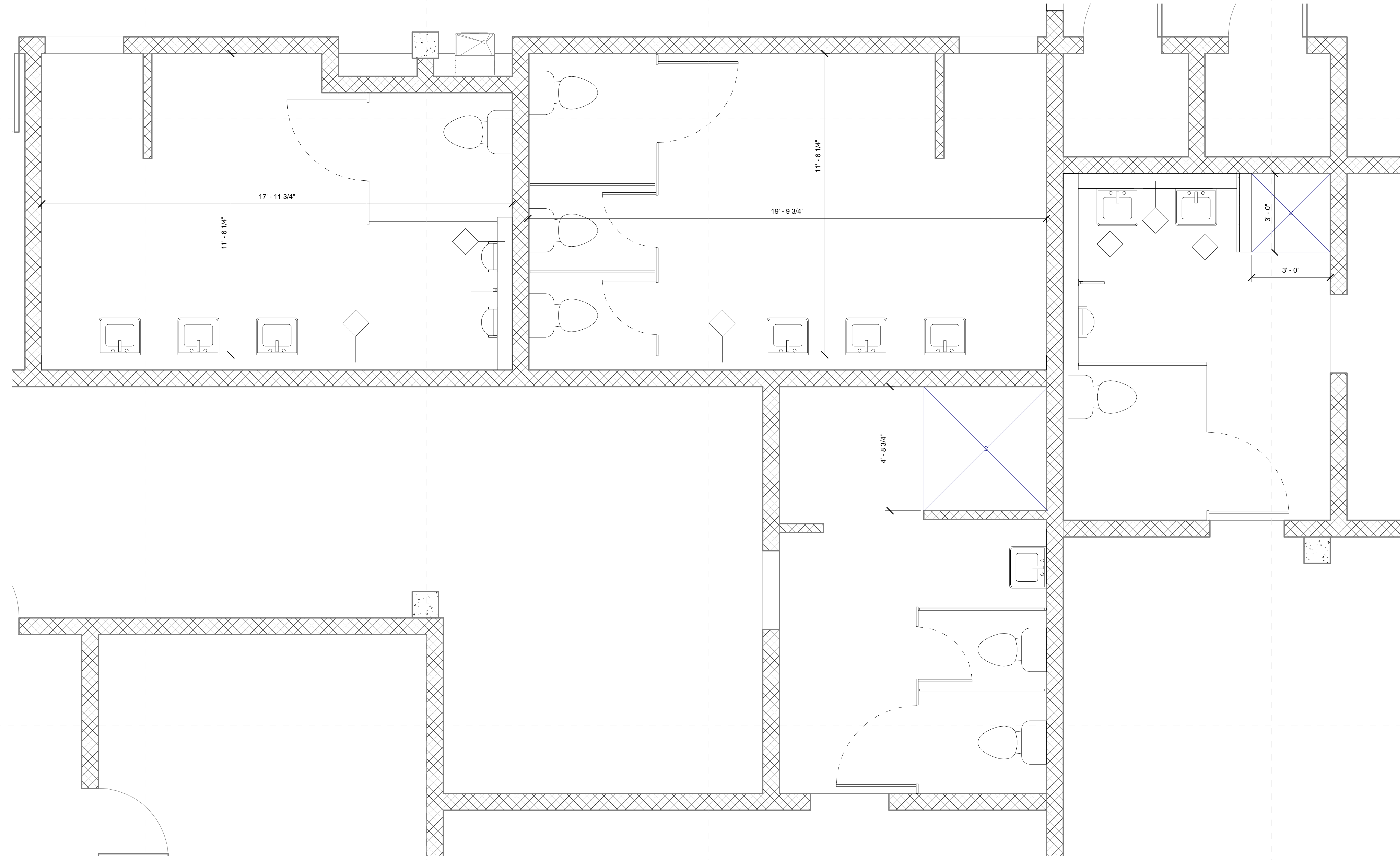
1 PCS Junior High 1st LVL - Bathrooms 1/2" = 1'-0"
