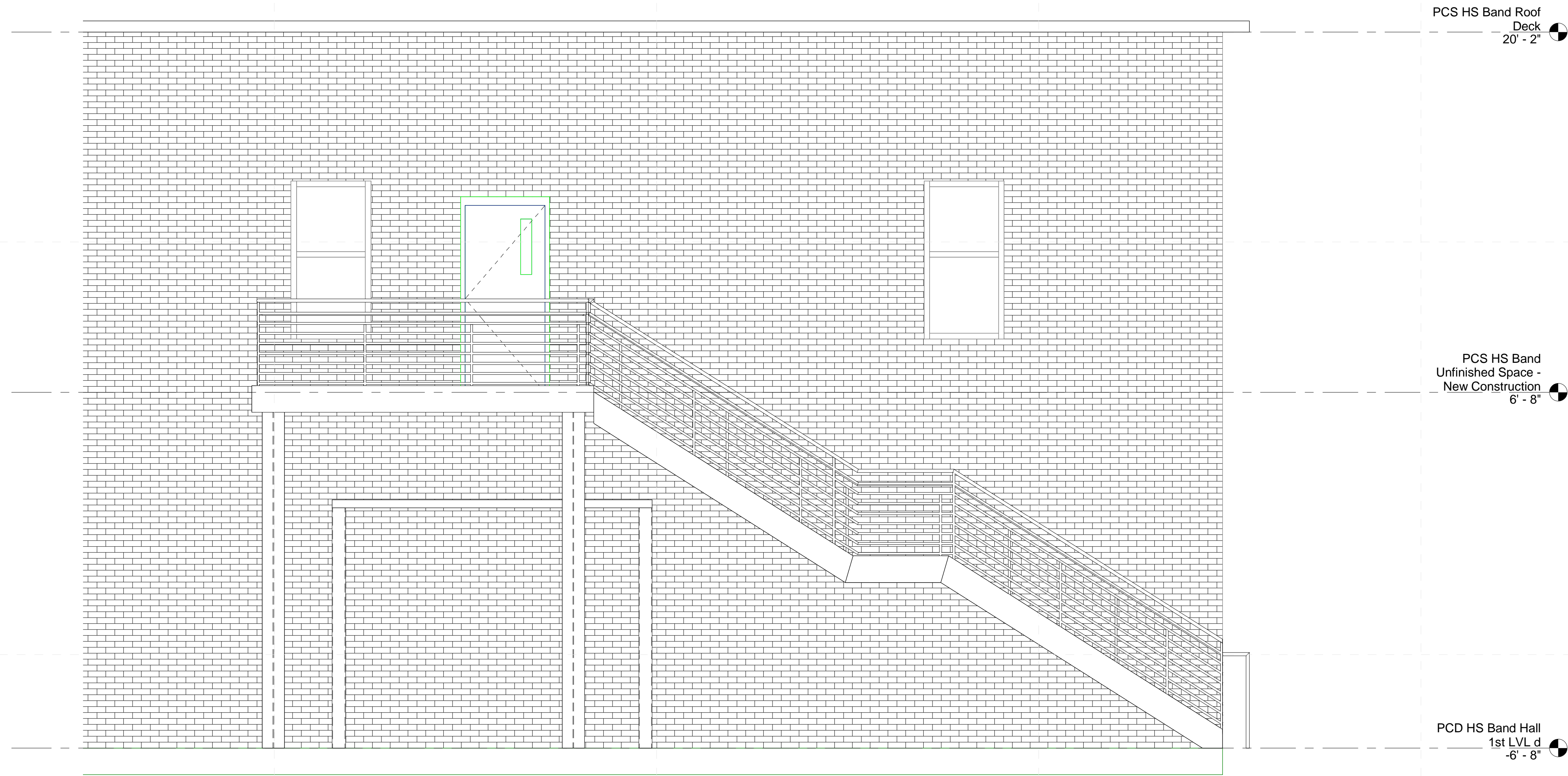
1 STAIR WALL 3/8" = 1'-0"
