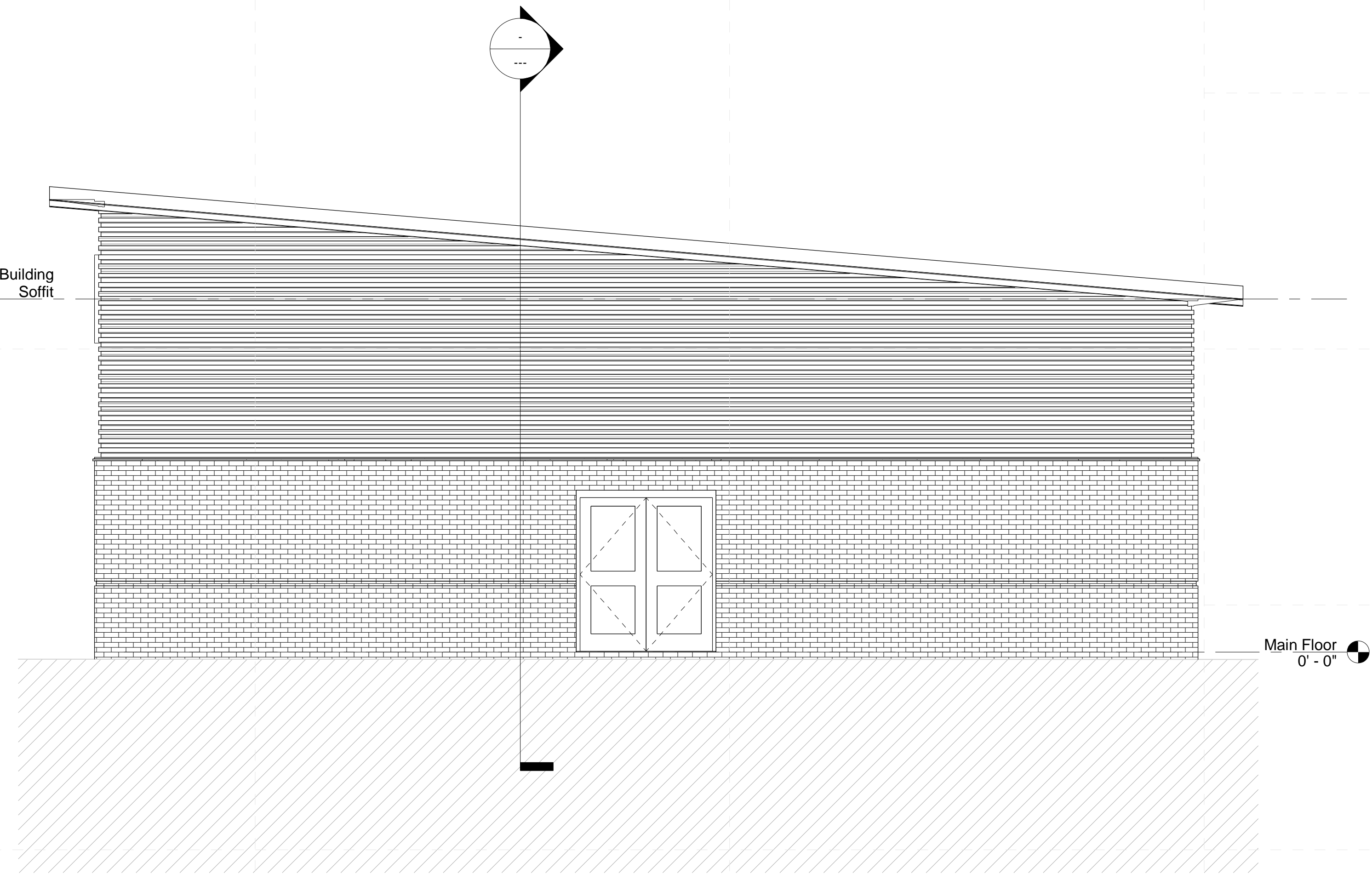
4 Multi Purpose Building South 1/4" = 1'-0"
