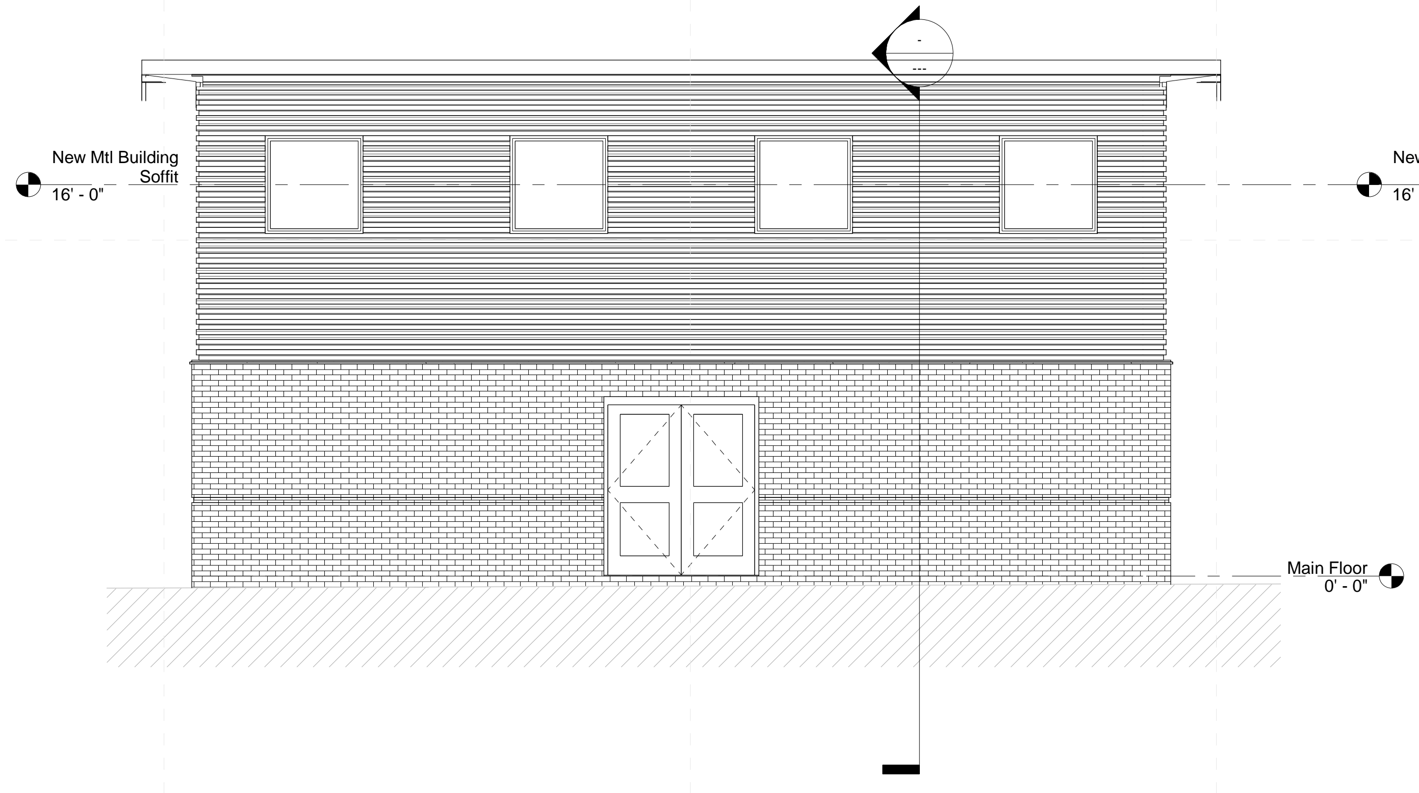
2 Multi Purpose Building West 1/4" = 1'-0"
