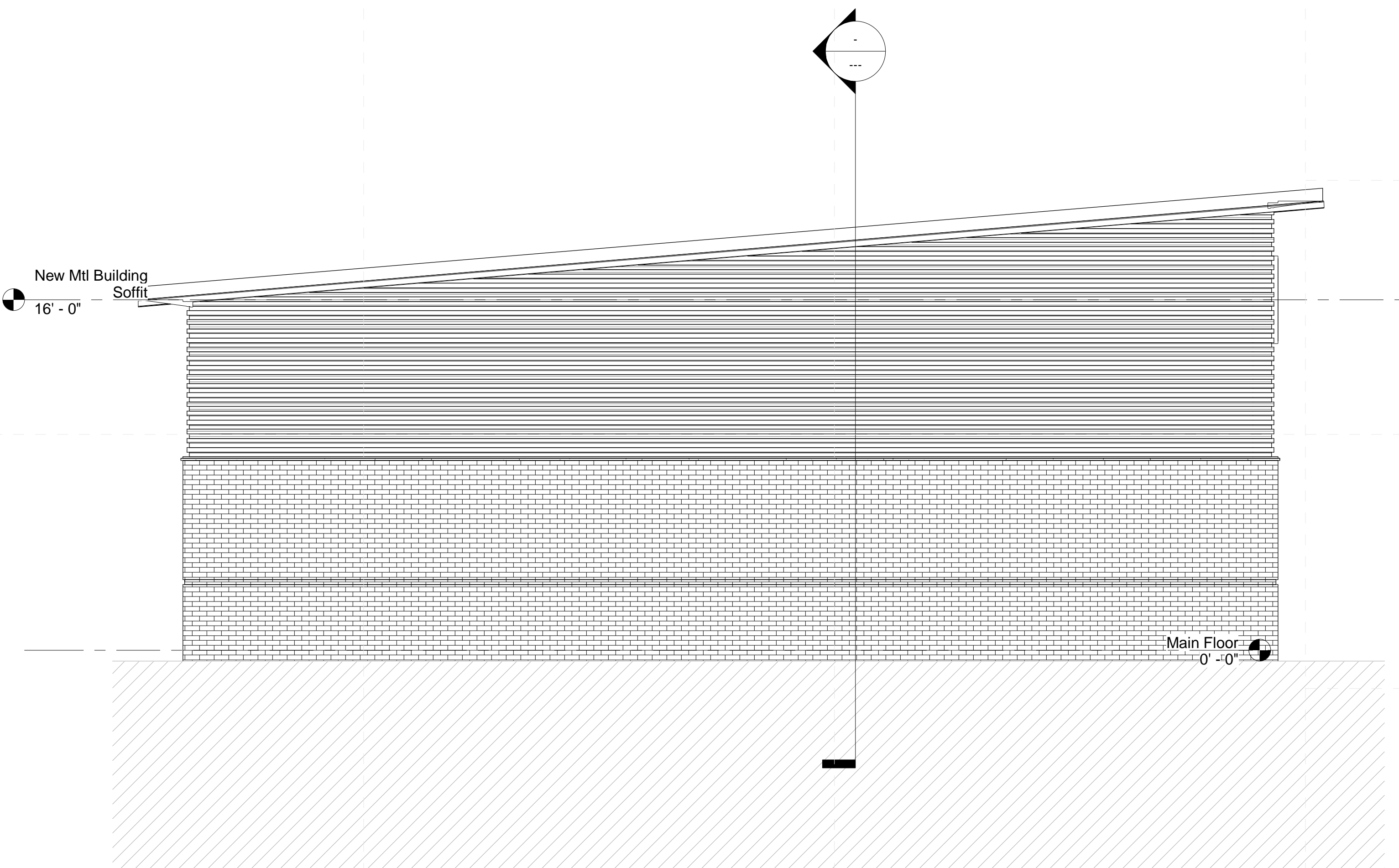
3 Multi Purpose Building North 1/4" = 1'-0"
