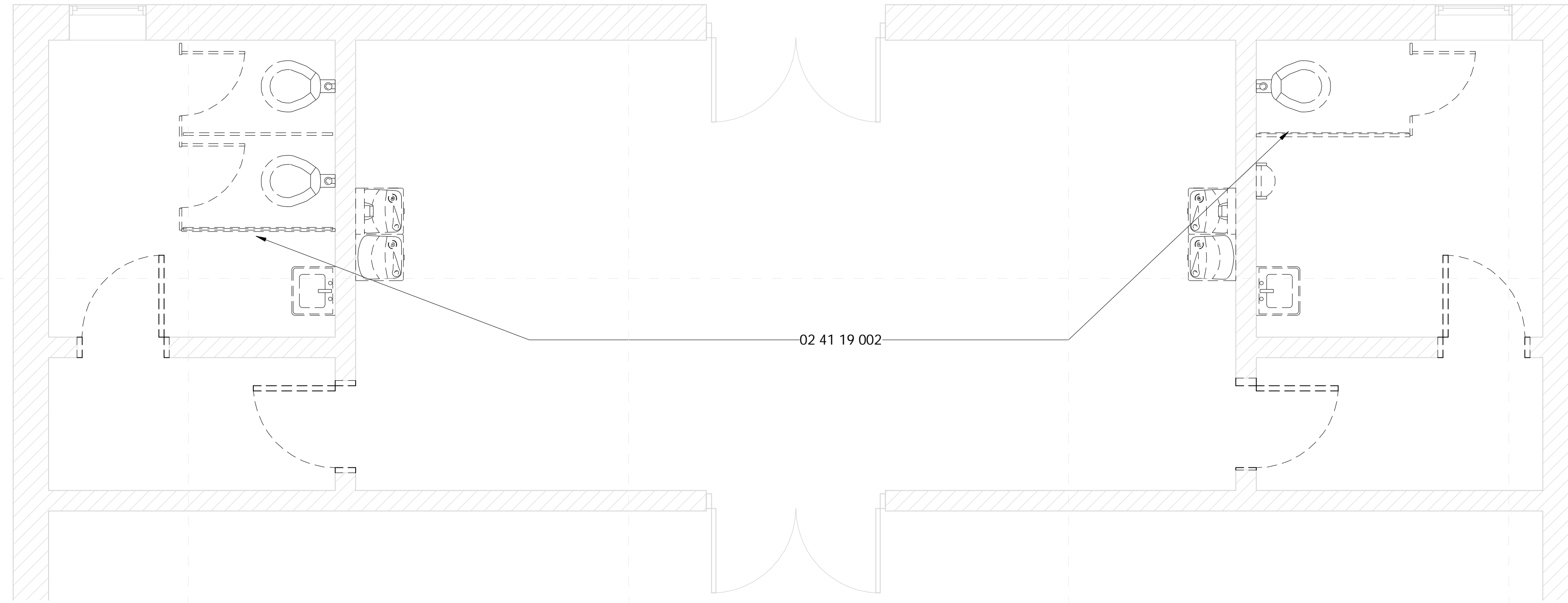
1 Toilets (Auditorium) - Demolition 3/8" = 1'-0"
