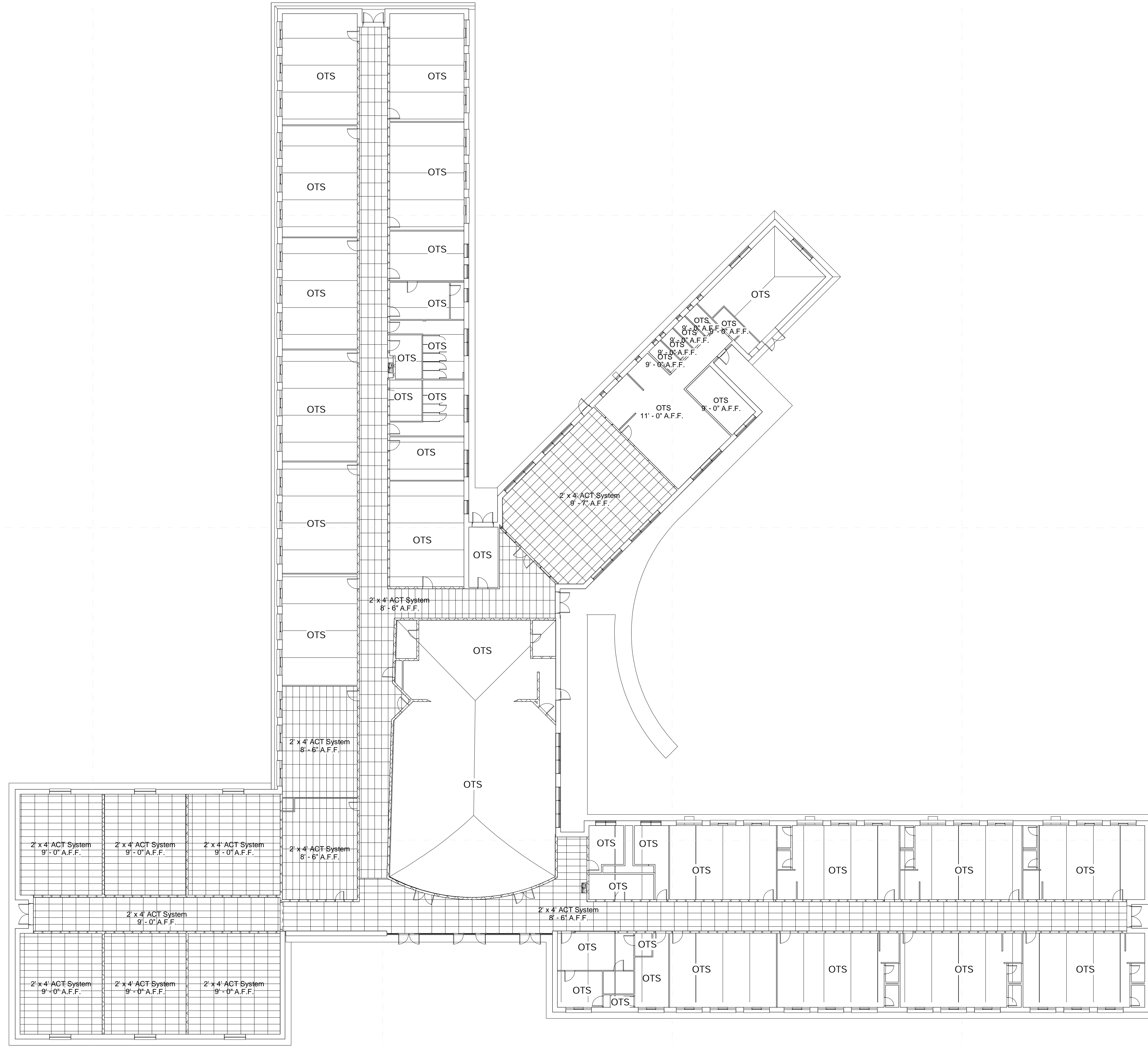
1 RCP - Demolition 1/16" = 1'-0"
