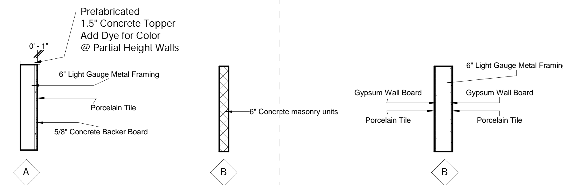
Wall Types
